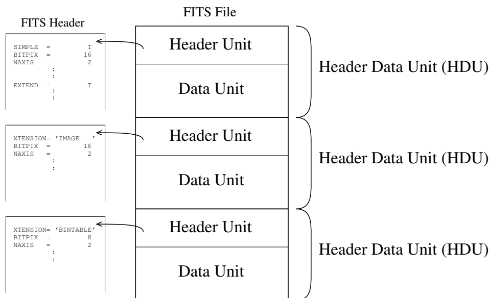
Figure 2: Overall structure of FITS file
