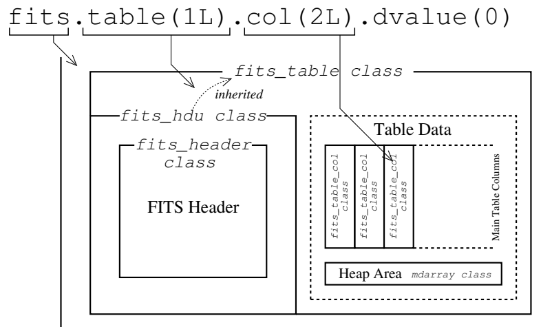
Figure 6: Detailed class structure of Binary Table HDU in Figure 4 and example API used to access cells in the Binary Table.
