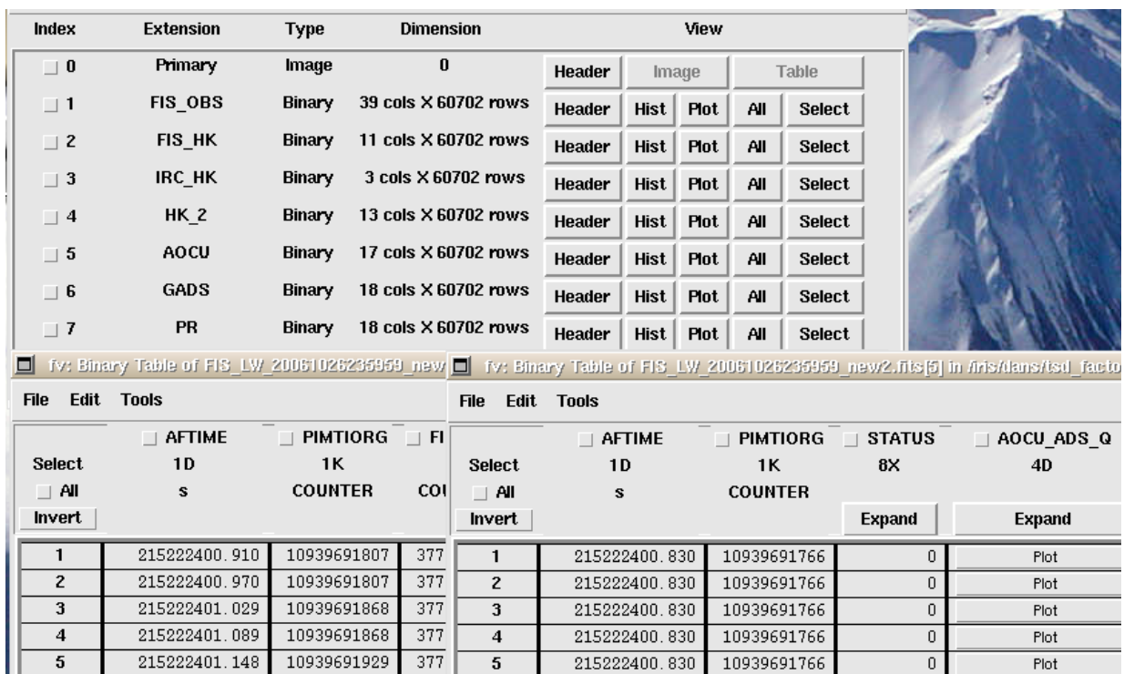
Figure 1: TSD, a standard data format used in software projects for “Akari”, the infrared astronomy satellite, can be opened using fv. All tables other than Primary are binary.
