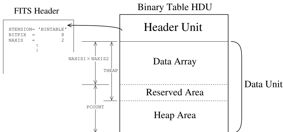
Figure 3: The structure of the Binary Table HDU. The size of each Data Unit can be determined from the values of NAXIS1 , NAXIS2 , PCOUNT , and THEAP . If there is no Reserved Area NAXIS1 × NAXIS2 will equal to THEAP and PCOUNT the size of the Heap Area.
