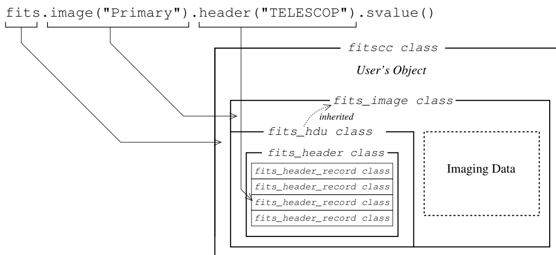
Figure 5: Detailed class structure of the Primary HDU in Figure 4 and example of API that accesses header records.
