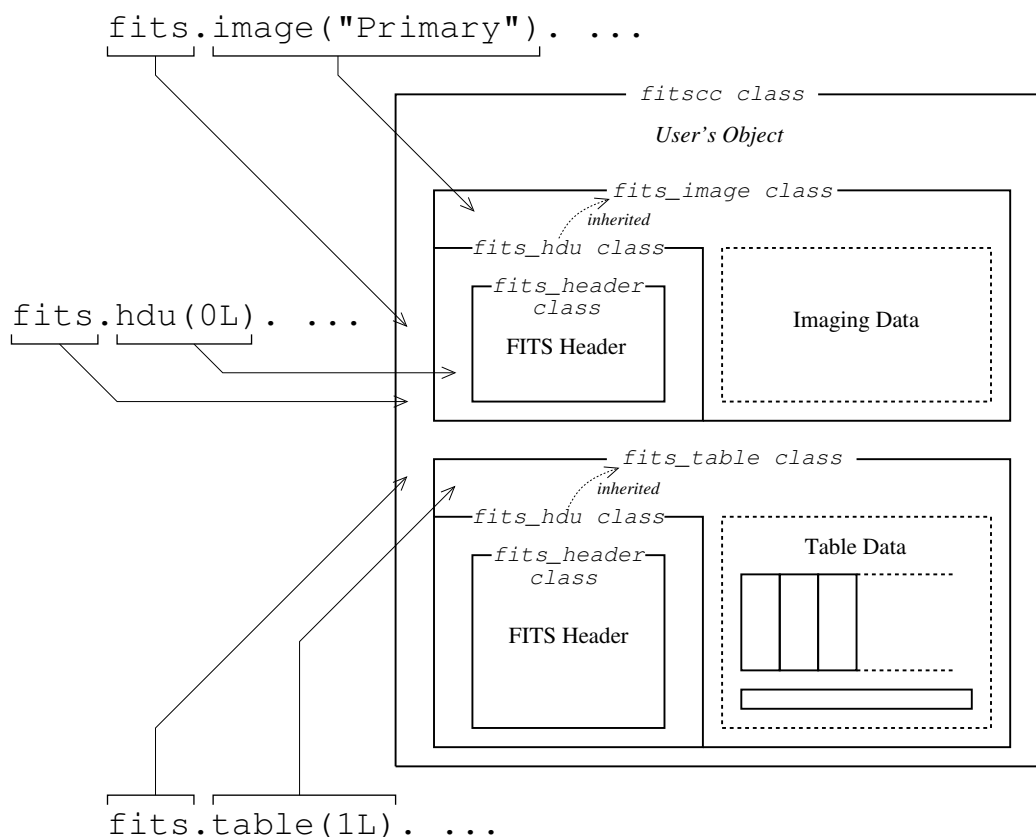
Figure 4: Overall internal structure of the object of “fitscc” class, which corresponds to one FITS file (right) and API that accesses each HDU (left). In this example one FITS file contains one Image HDU and one Binary Table HDU.
